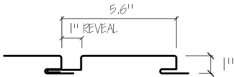
5 PANEL PROFILE NTS
