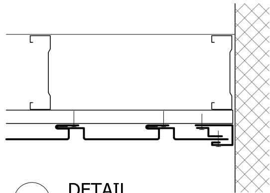
3 DETAIL NTS
