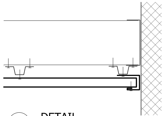
4 DETAIL NTS
