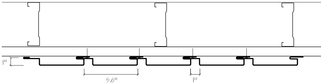
1 SECTION NTS
