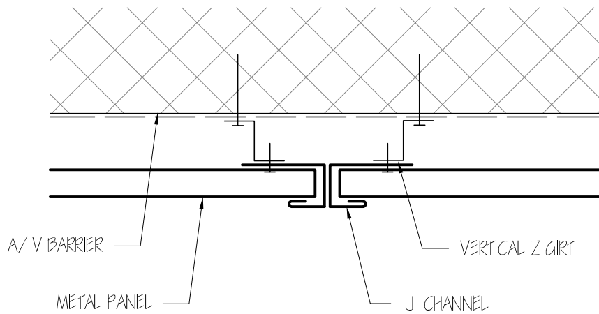
4 HORIZONTAL JOINT DETAIL NTS
