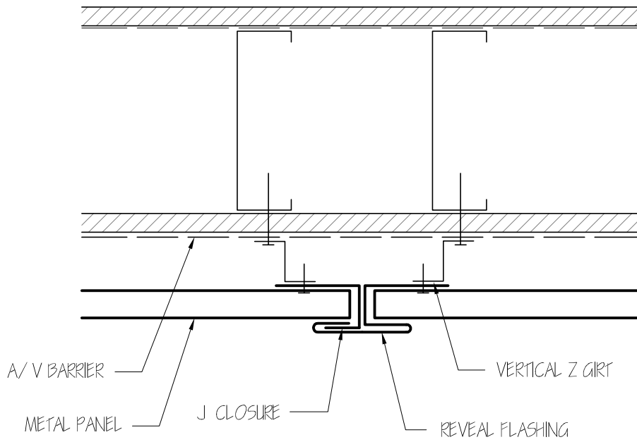
3 HORIZONTAL JOINT DETAIL NTS
