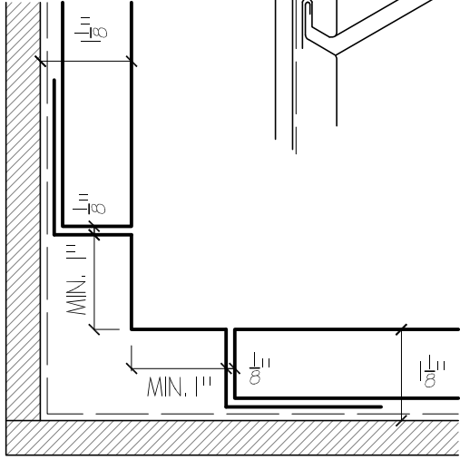
1 INSIDE CORNER DETAIL NTS
