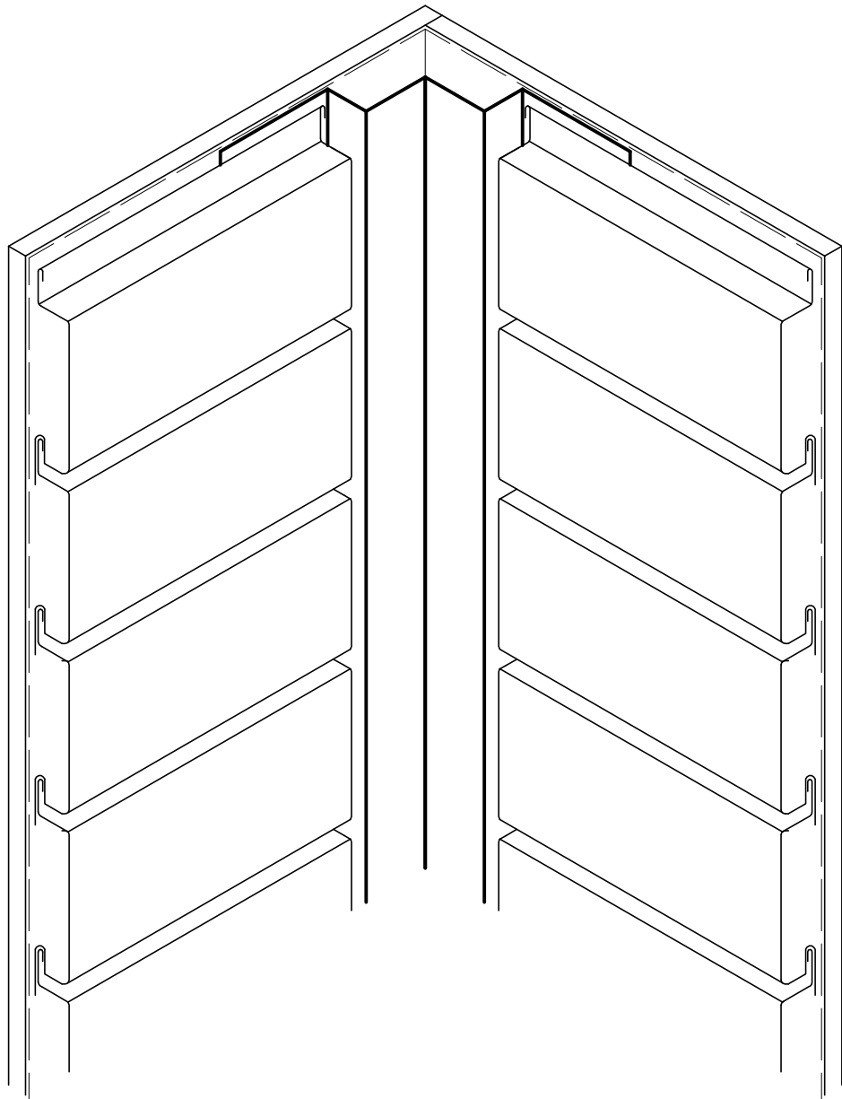
1 INSIDE CORNER DETAIL NTS
