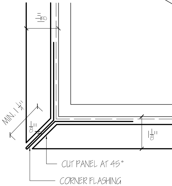
3 OUTSIDE CORNER DETAIL NTS
