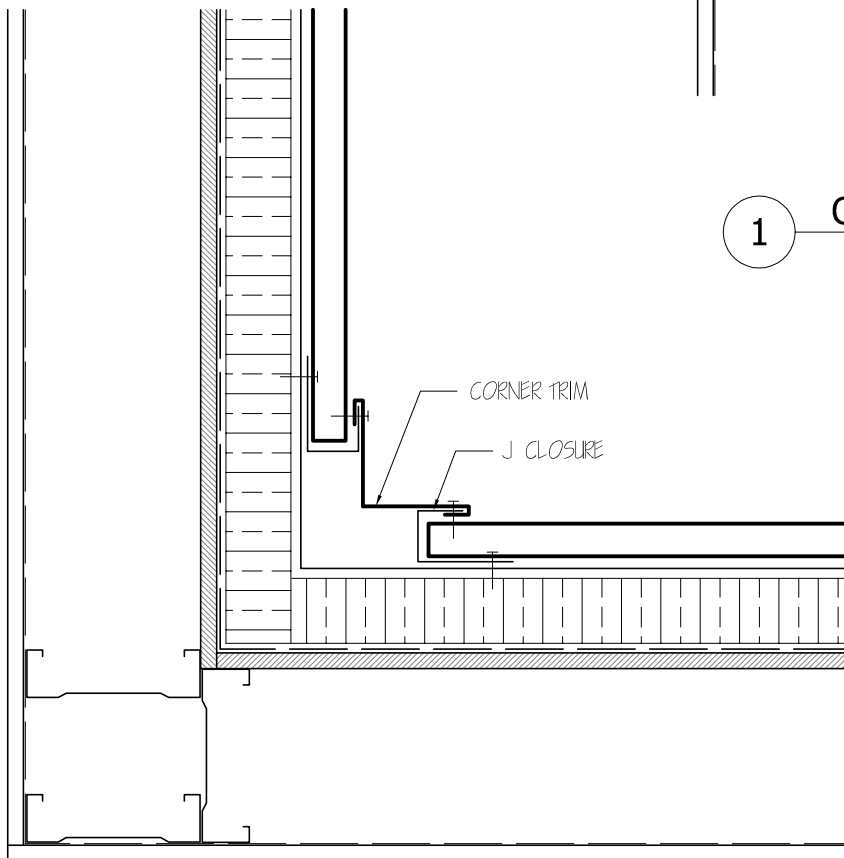
2 INSIDE CORNER DETAIL NTS
