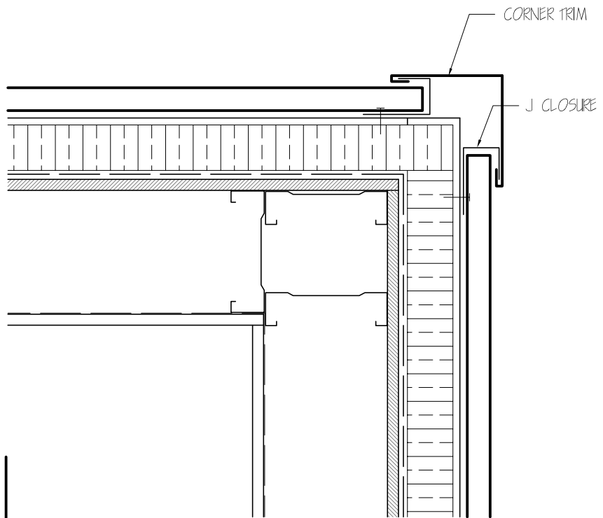
1 OUTSIDE CORNER DETAIL NTS
