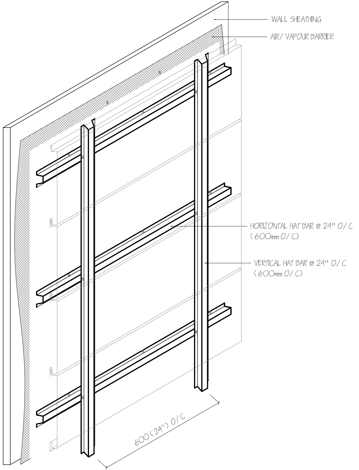
2 UNINSULATED SUB-GIRT SYSTEM NTS
