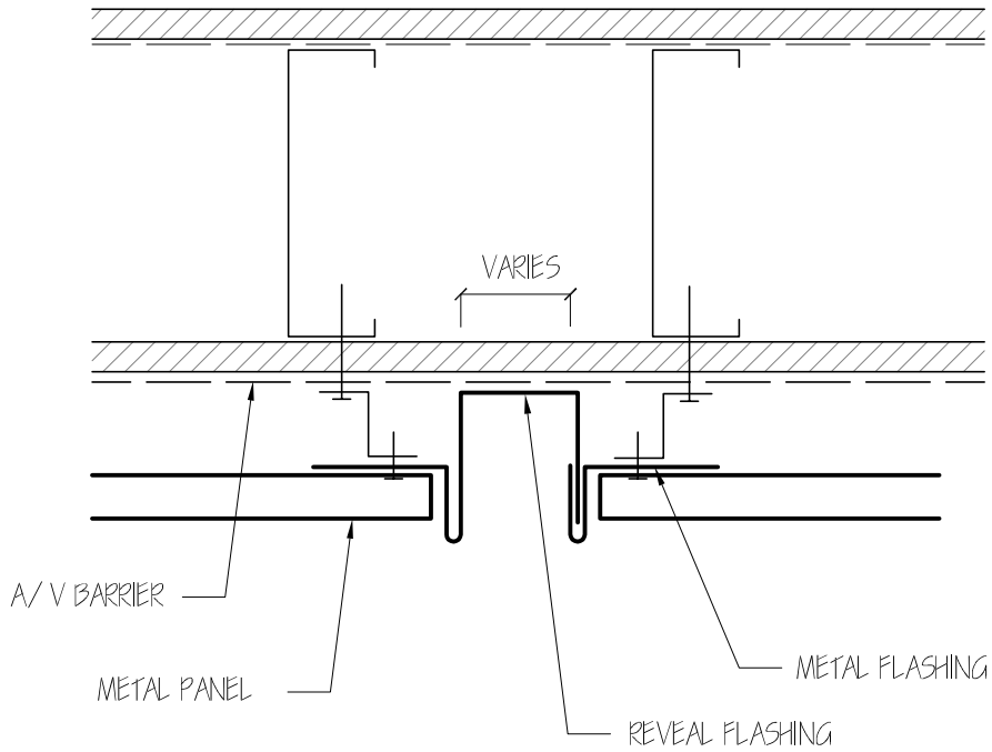
1 HORIZONTAL JOINT DETAIL NTS
