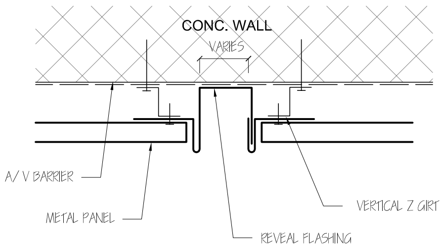
2 HORIZONTAL JOINT DETAIL NTS
