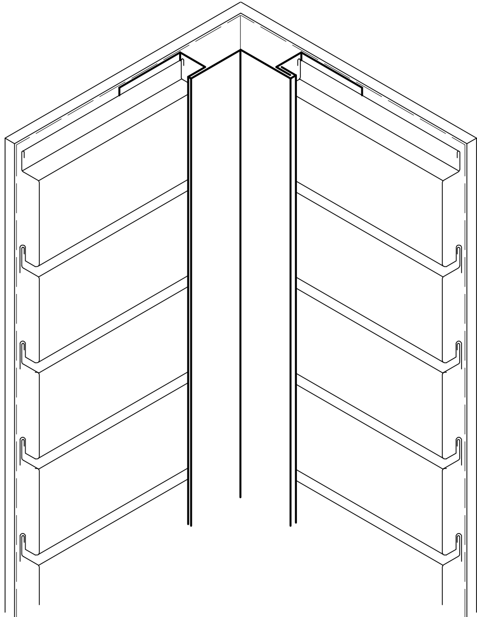
2 INSIDE CORNER DETAIL
