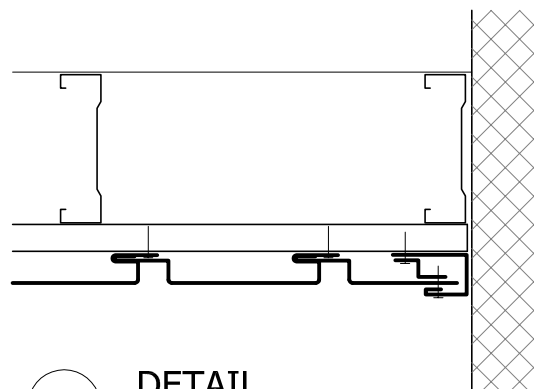
3 DETAIL NTS
