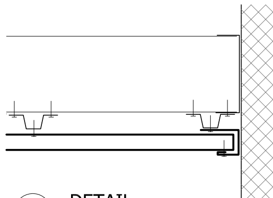
4 DETAIL NTS
