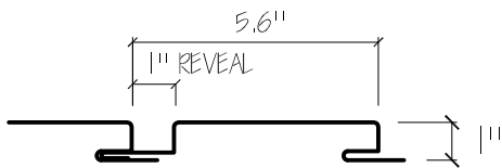
5 PANEL PROFILE NTS
