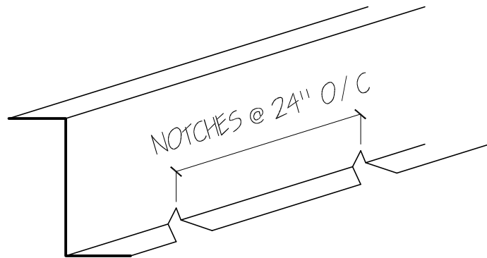
Z GIRT DETAIL
