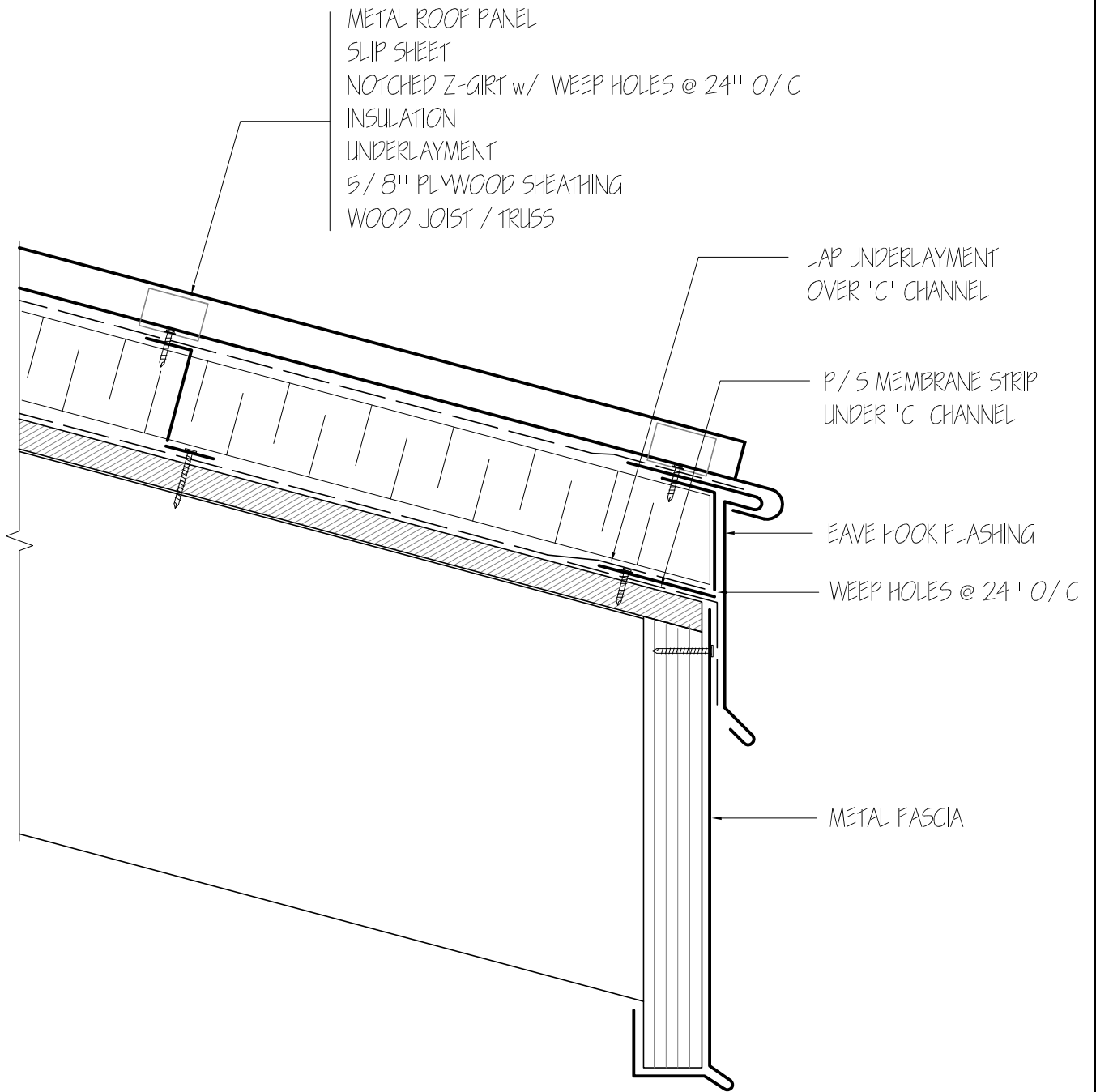
1 TYPICAL EAVE DETAIL (INSULATED ROOF SYSTEM)
